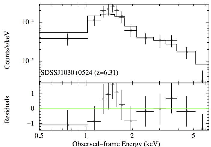
Fig. 4: X-ray spectrum of SDSS J1030+0524 fitted with a power-law model ( \Gamma = 1.81^{+0.18}_{-0.18} ). In the bottom panel we report the residuals [(data–model)/error]. For display purposes we adopted a minimum binning of ten counts per bin.
