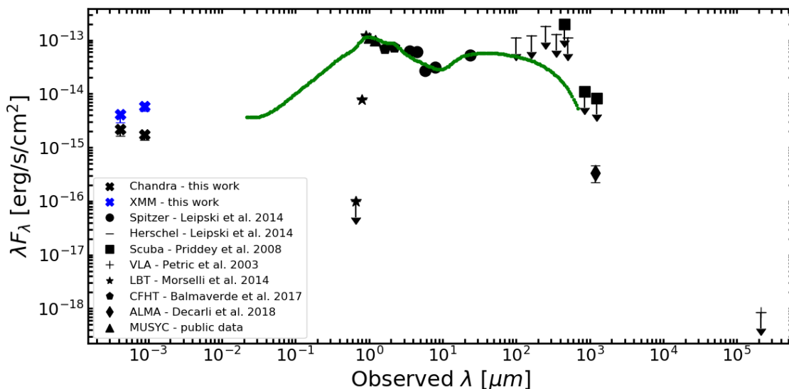
Fig. 9: Multi-wavelength SED of SDSS J1030+0524. References to the points are labelled. The green curve is the combined SED for luminous lower redshift QSOs taken from Richards et al. (2006)
