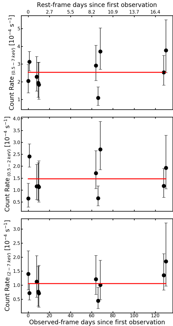
Fig. 2: Count rate of SDSS J1030+0524 in the three X-ray bands (full in the top, soft in the middle, and hard in the bottom panel) extracted from the ten Chandra observations vs the days since the first observation. Errors are reported at the 1\sigma level. The red solid lines represent the weighted mean.
