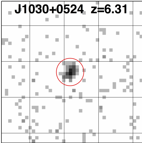
Fig. 1: Full-band (0.5 – 7 keV) Chandra ACIS-I image of SDSS J1030+0524. The red circle represents our extraction region (2'' radius). The grid separation is 5'' and the cutout spans 20''x20'' on the sky.
