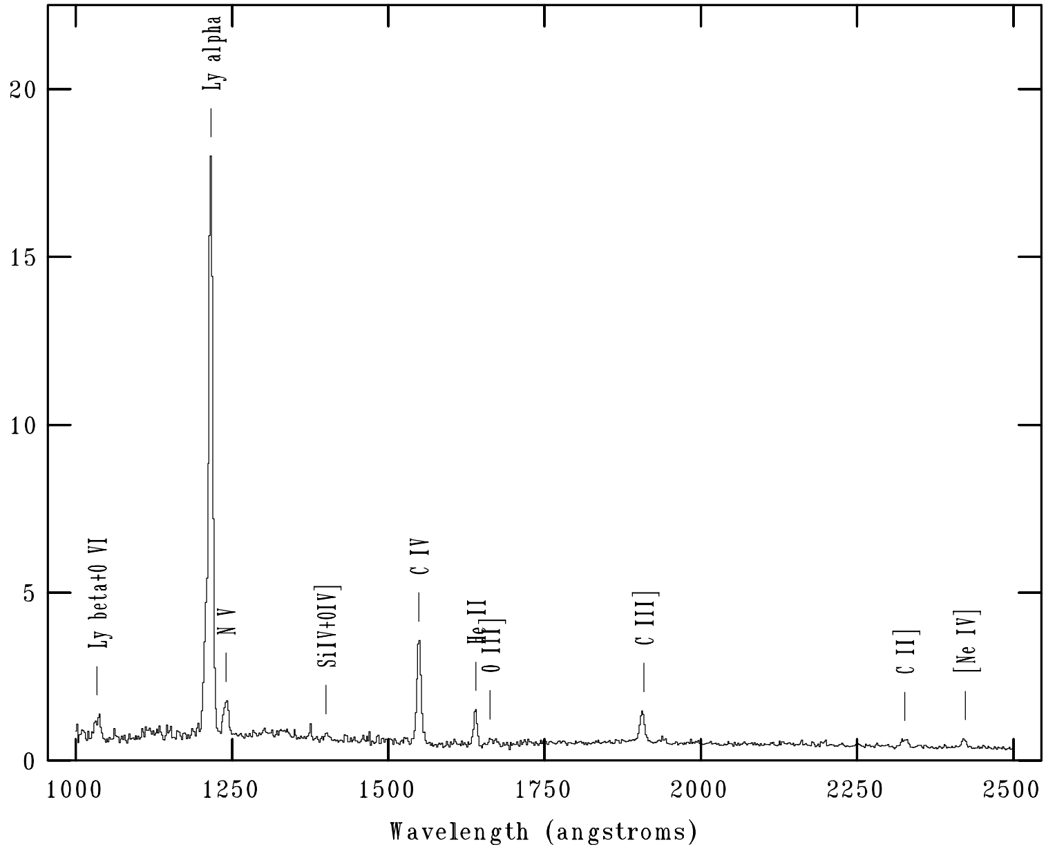
r.m.s. spectrum of Composite type 2 AGN
